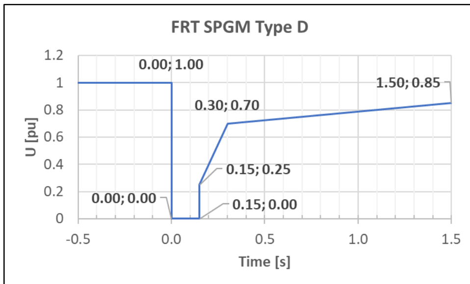
Figure 4.21 Fault-ride-through profile of a type D SPGM
