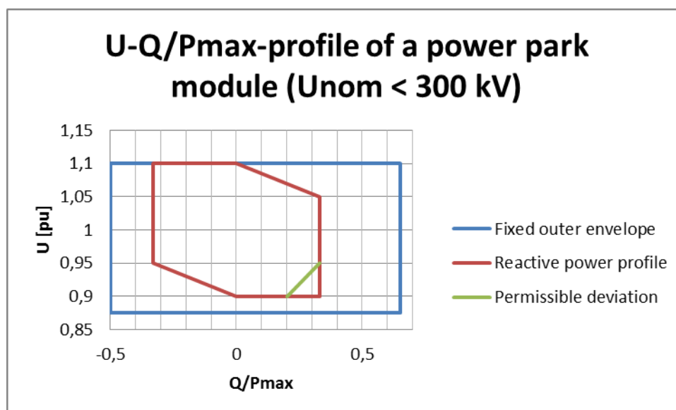
Figure 4.13 U-Q/P max profile of a power park module Type B and Type C and Type D (U nom < 300 kV)
