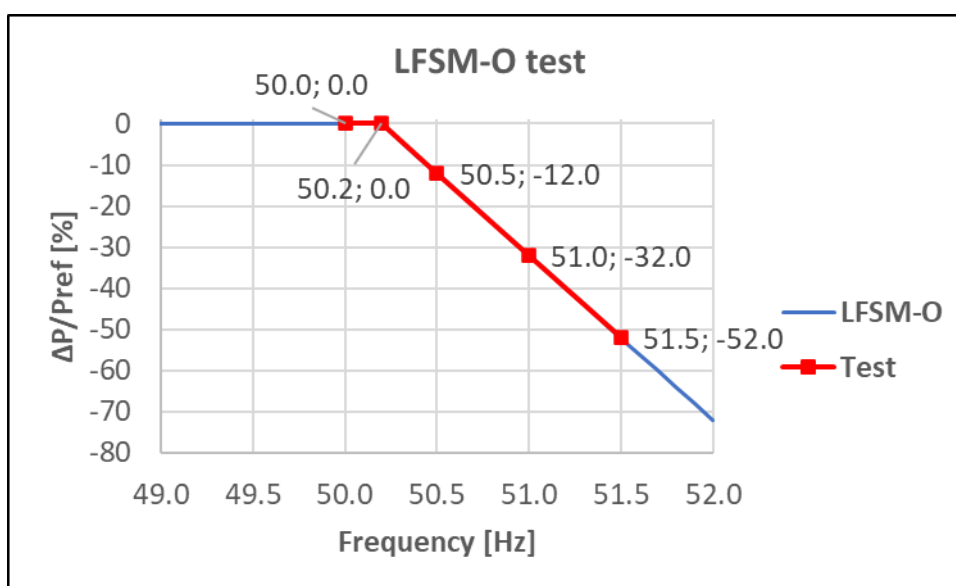
Figure 4.5 LFSM-O test points corresponding to 5% droop
