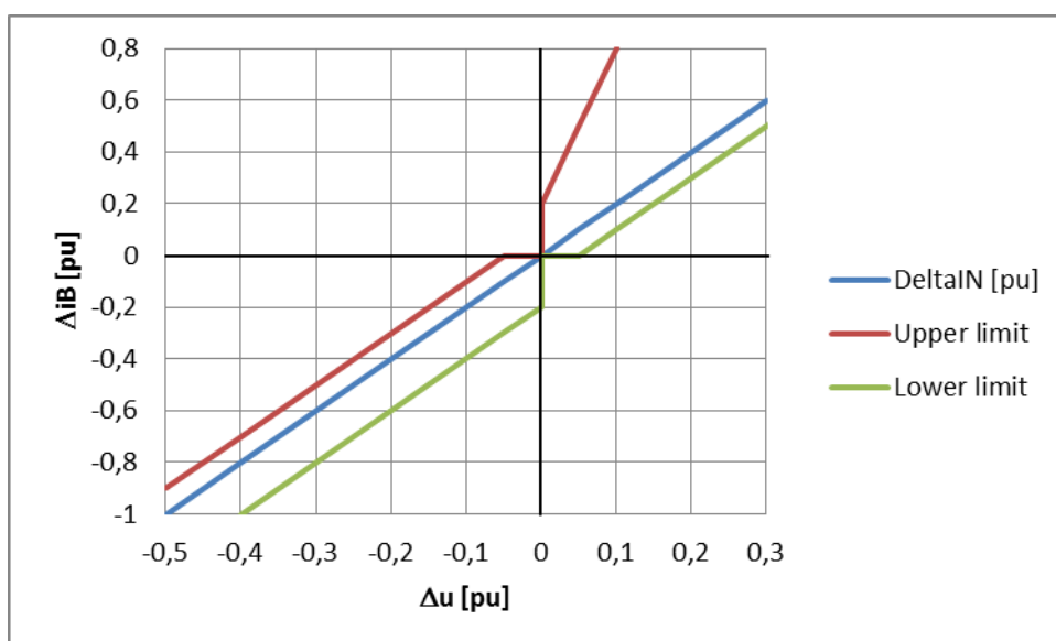
Figure 25 Additional reactive current injection; example for k=2 and tolerances
