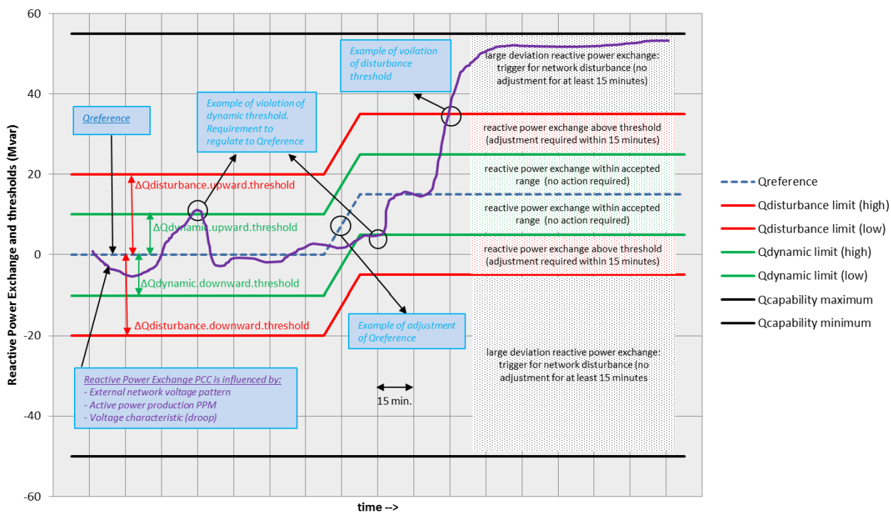
Figure 4.18 Example of Reactive Power Exchange of a Generator or (O)PPM at the PCC and Reactive Power thresholds in Voltage control mode sub-mode 1
