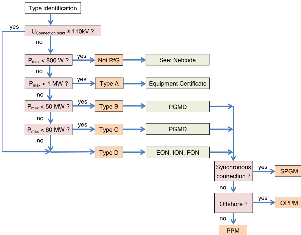
Figure 3.1 RfG Type identification
