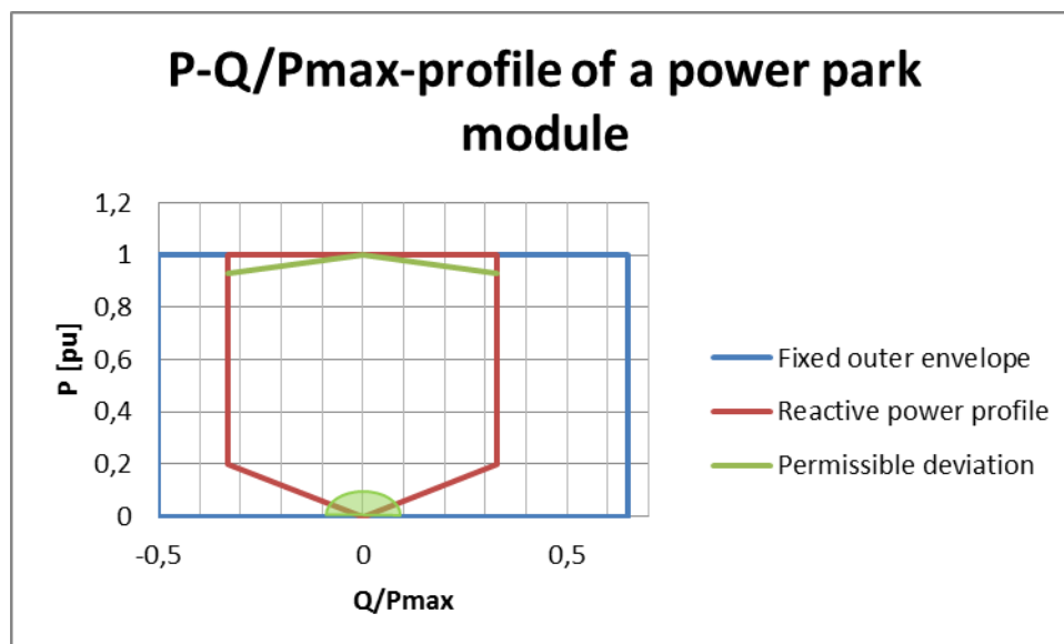
Figure 4.14 P-Q/P max profile of a power park module Type B and Type C
