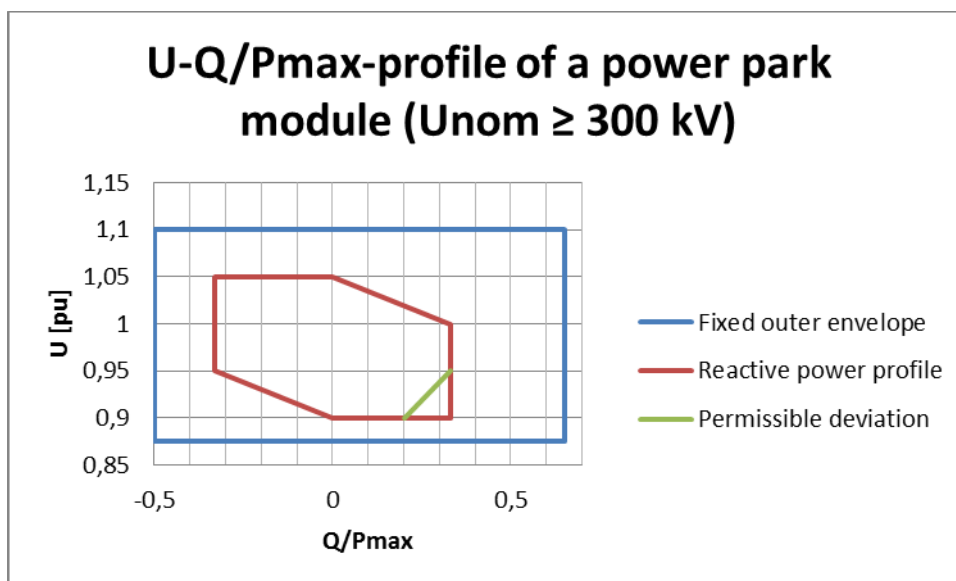
Figure 4.15 U - Q/P_{max} profile of a power park module Type D (U nom ≥ 300 kV)
