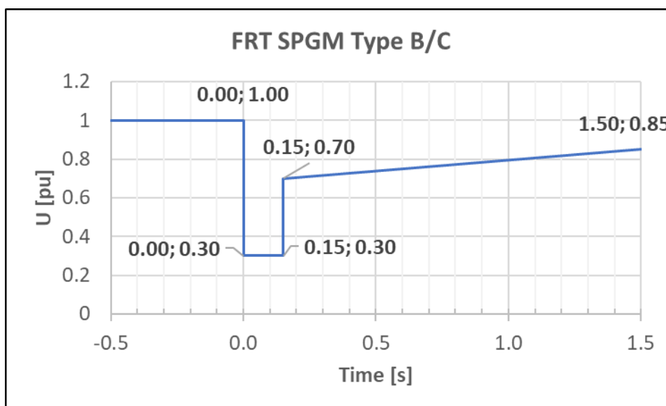
Figure 4.19 Fault-ride-through profile of a type B/C SPGM
