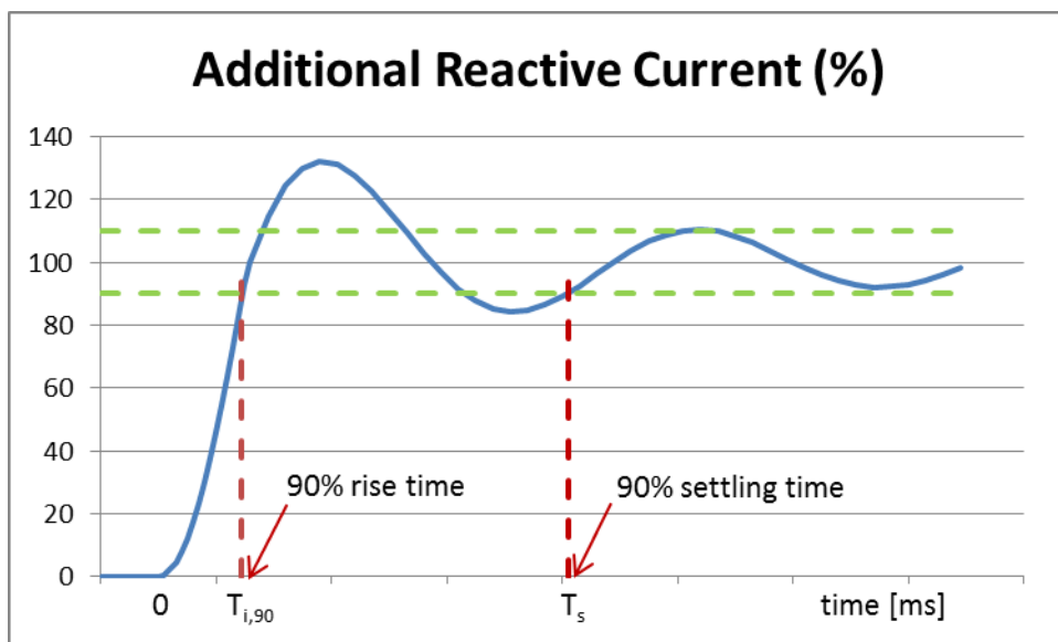
Figure 24 Additional reactive current step response
