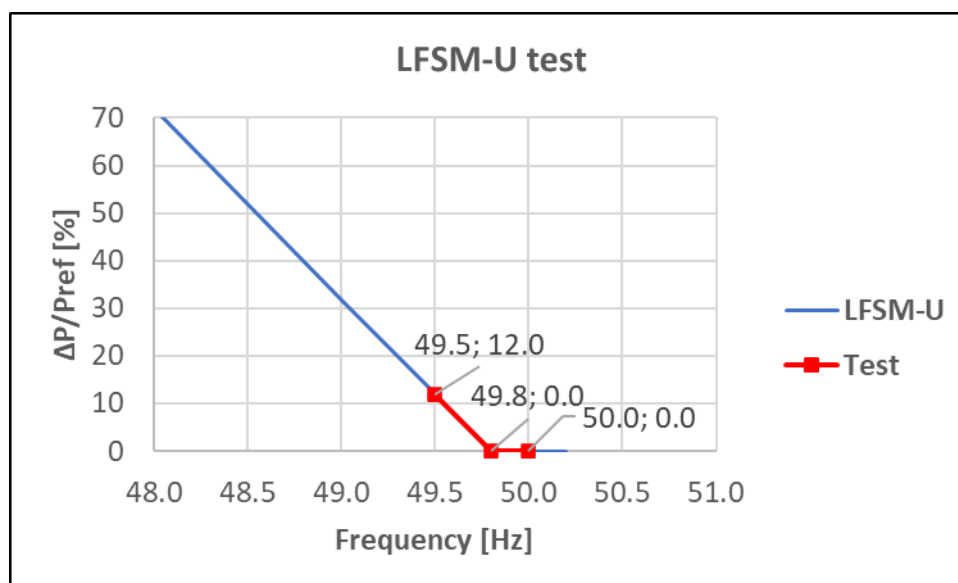
Figure 4.7 LFSM-U test points corresponding to 5% droop
