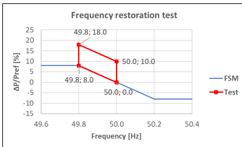
Figure 4.11 Frequency restoration test points corresponding to 5% droop
