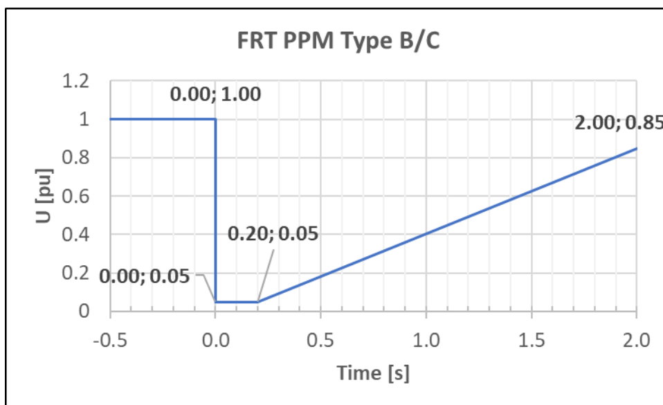
Figure 4.20 Fault-ride-through profile of a type B/C PPM
