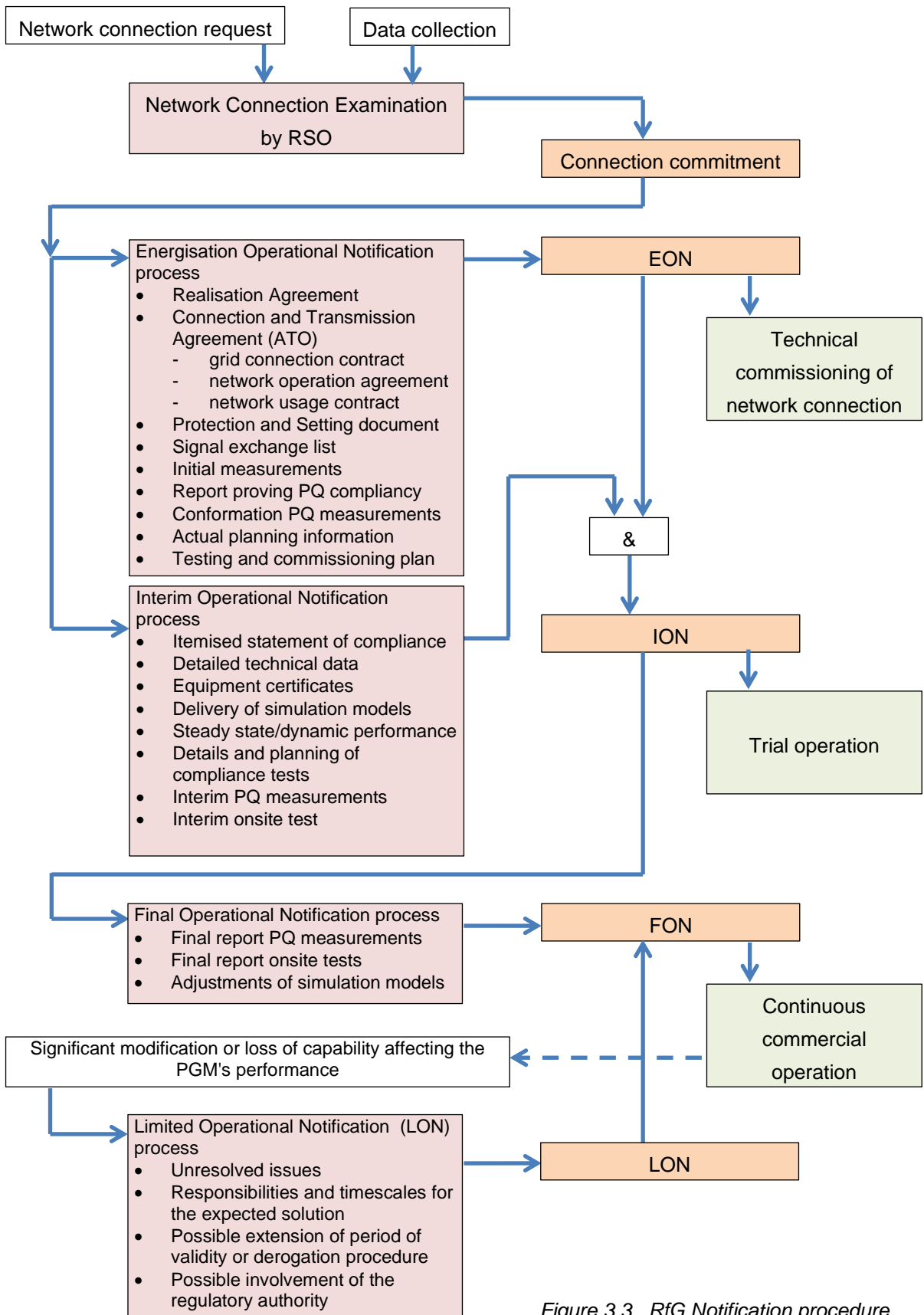
Figure 3.3 RfG Notification procedure
