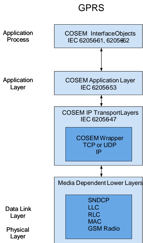
Figure 3.2: GPRS communication profile
