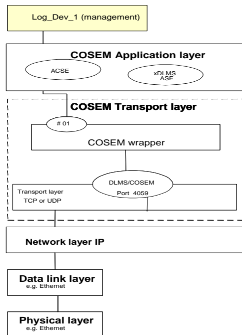
Figure 3.1: TCP/UDP based profile
