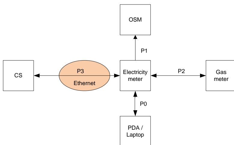
Figure 1.2: DLMS/COSEM infrastructure P3
