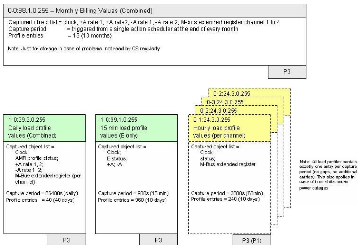
Figure 4.1: Structure of profiles of Dutch Smart Meter
